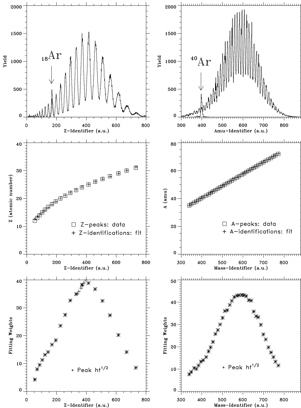
Figure 9.8: Lower-energy run. Top row: One-dimensional projections from 2D Z -identifiers and A -identifiers shown in Fig. 9.5, with ^{40}_{18}\text{Ar} cyclotron-analog calibration beam overlaid to illustrate particle identifications. Middle row: Fits to centroids of Z - and A -identifiers' peak locations. Bottom row: Statistical weights used in multiple-peak fitting to Z - and A -identifiers' peaks.
